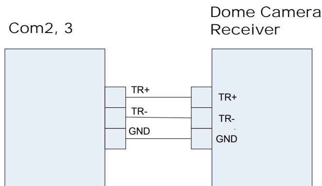
COM2/COM3 diagram (RS-485)
