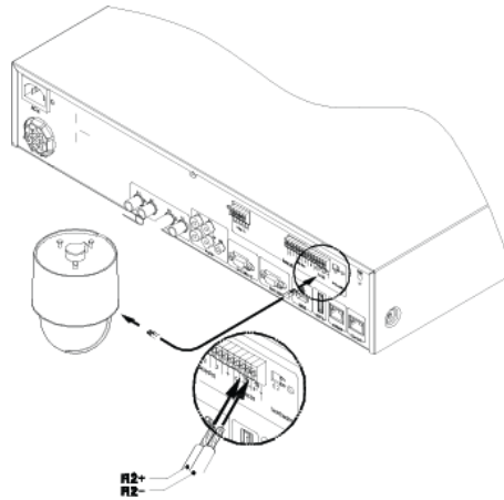
Serial communication port diagram COM1 connection diagram (RS-232 – D-Sub)
