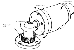
Figure 2-3 3-axis Adjustment
